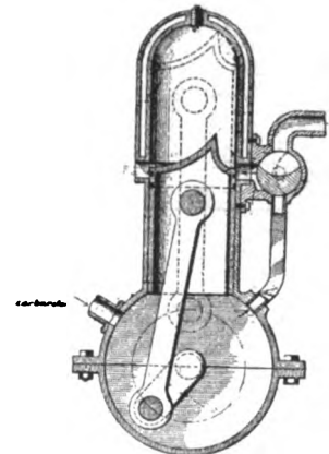
Snyder Rotary Valve Engine.
